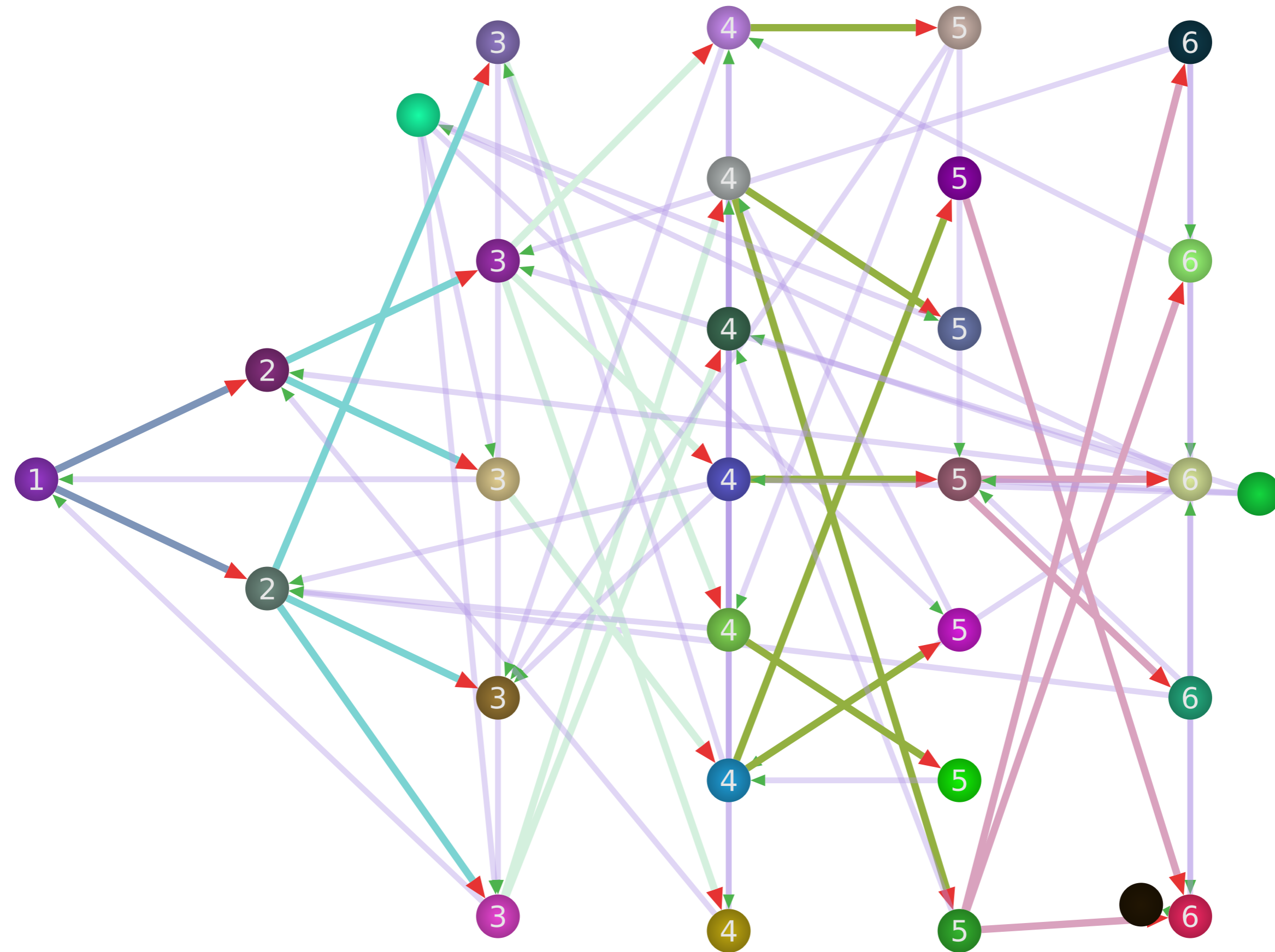
The presentation of a breadth-first search in a directed graph
